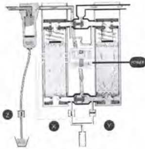
Figure 7.2. Dryer in operation
